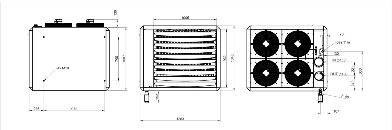
Figure 5 - Dimensions TRX+117
