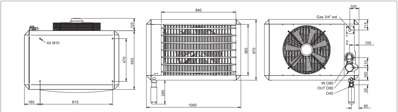
Figure 3 - Dimensions TRX+55 - TRX+65
