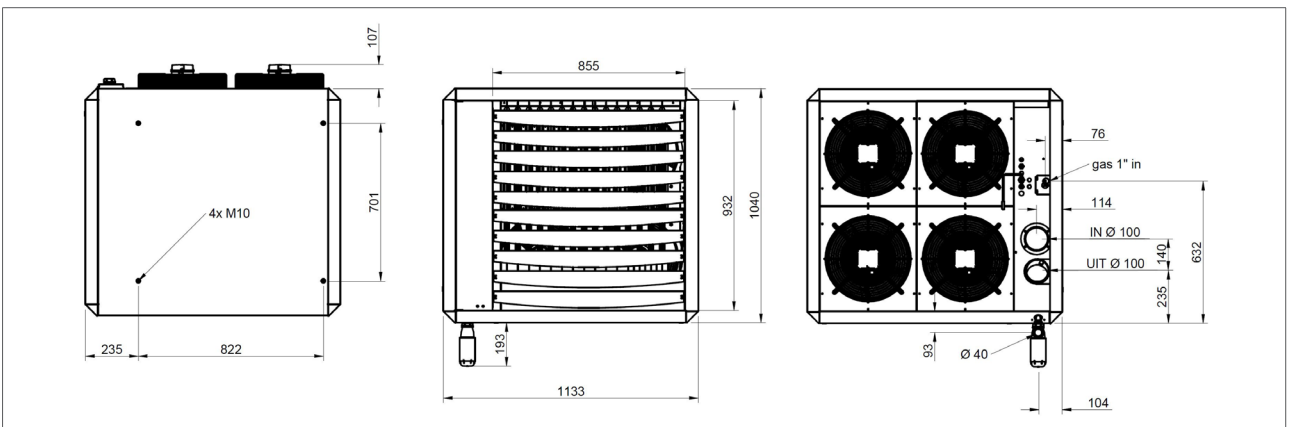
Figure 4 - Dimensions TRX+78 - TRX+97
