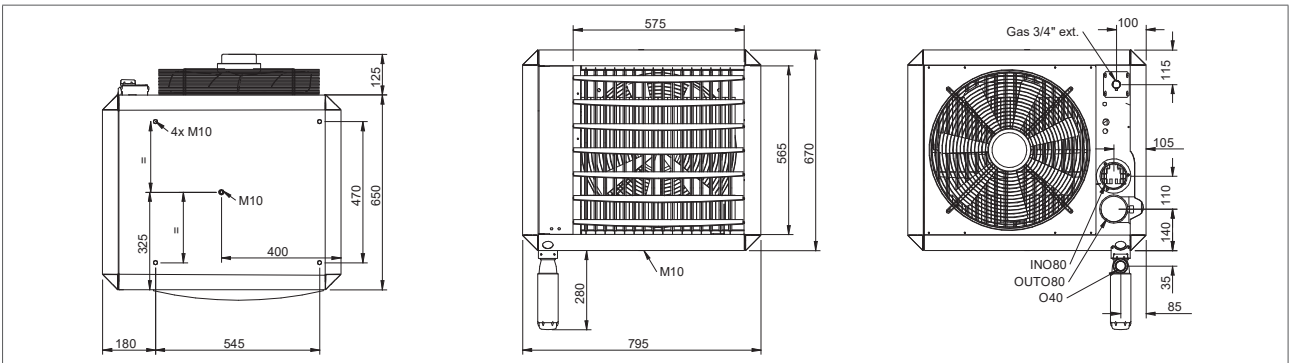
Figure 2 - Dimensions TRX+32 - TRX+44
